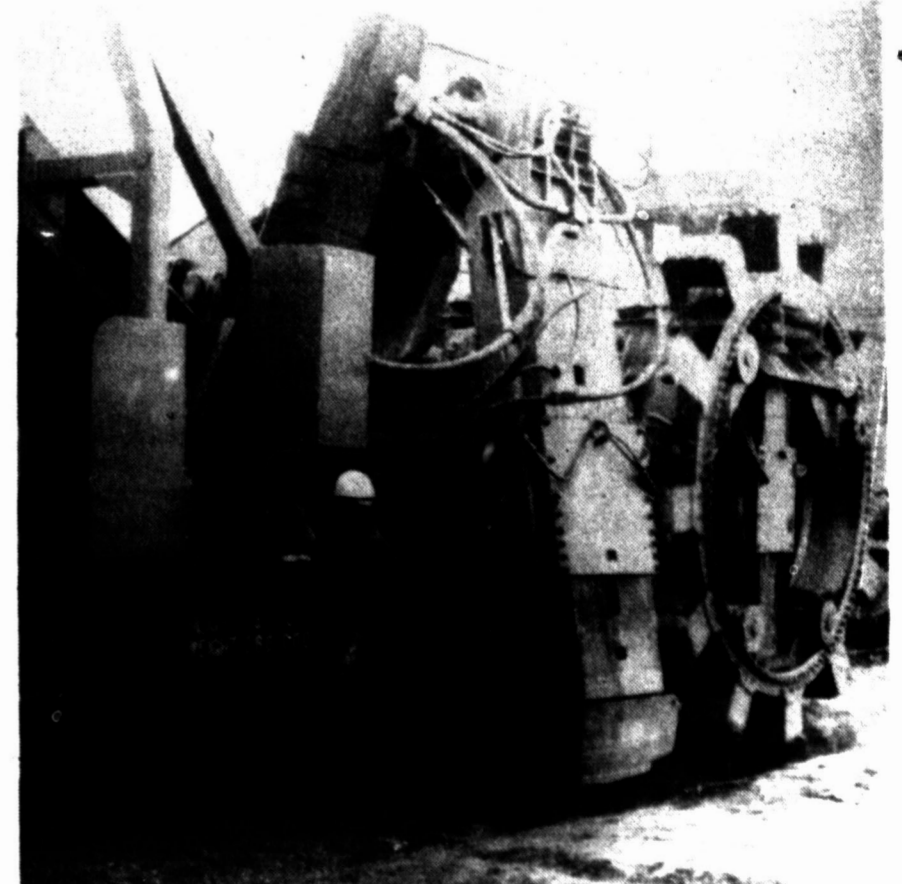
EXPENSIVE MACHINE working on the track in the old Fort Worth and Denver right-of-way in Clarendon. The machine cuts away soft dirt under the ties so that it can be replaced with firm crushed rock.
