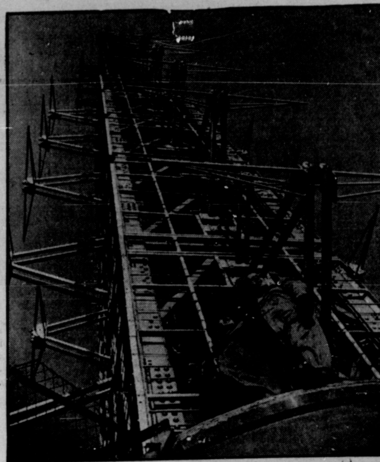
VIDEOZONE —High above New York City, two radio experts hold a conversation at the base of the Empire State Building television antenna mast. Final grid—last large structural piece to be added to the tower, completing it except for wiring—when installed, should make the video antenna ready for broadcasting early in December, 1951.
