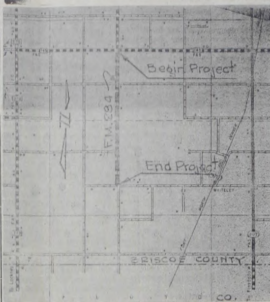
LEGEND: PARTIAL MAP OF BRISCOE COUNTY - FM ROAD 284 FROM FM 145, SOUTH TO ROAD INTERSECTION
