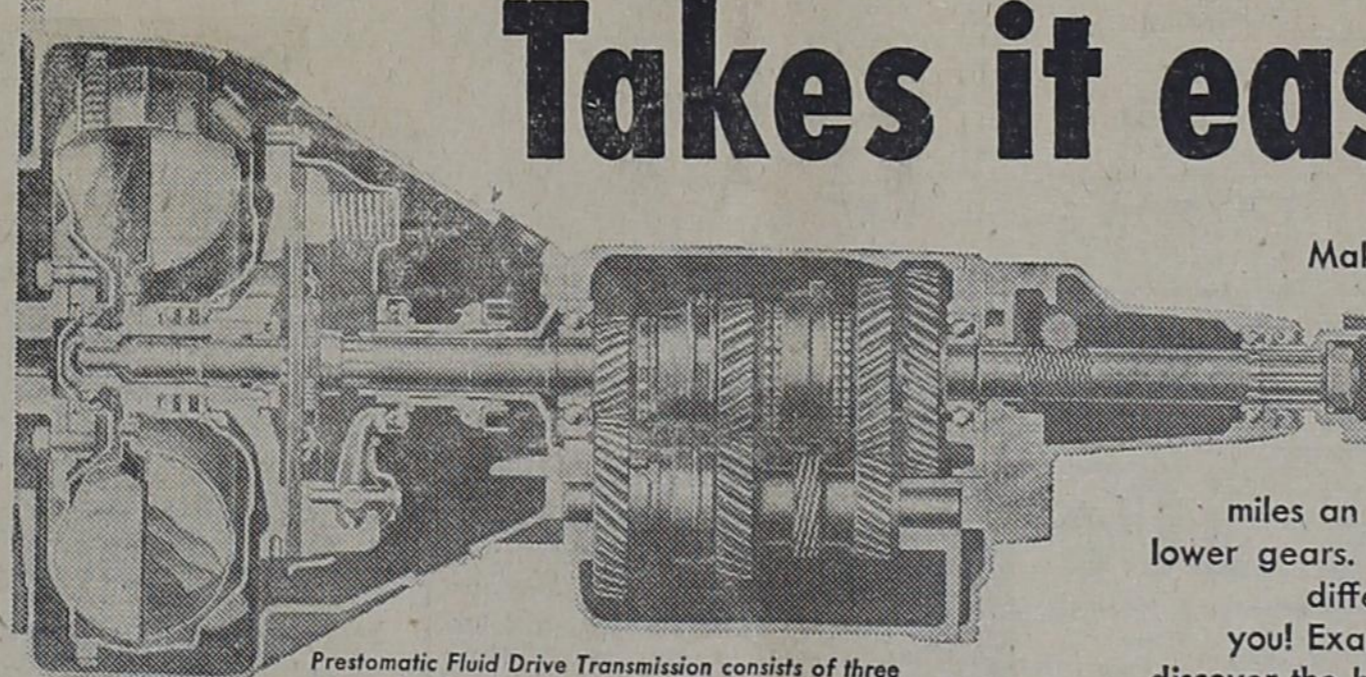
Prestomatic Fluid Drive Transmission consists of three compact units... the Safety Clutch and Prestomatic Transmission. Each unit is designed with a minimum of moving parts, and each unit is ruggedly built to give trouble-free service for the lifetime of the car.
