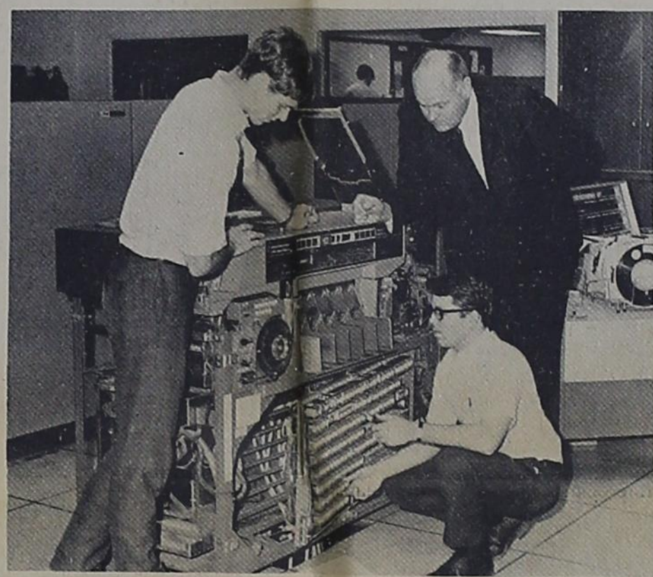
COMPUTER SAVINGS — Texas Tech electrical engineering students Harry Tredennick, left, and Kenneth Smith, son of Mr. and Mrs. J. Weldon Smith of Munday, discuss their modification of an IBM 088 collator to make it take on the additional function of a card reader, a $55,000 job done for less than $1,200 in parts. These students and one other, John Guest, made the conversion, working with Electrical Engineering Instructor A. F. Adkins, right, Prof. Darrell L. Vines and Computer Services Director George S. Innis.
