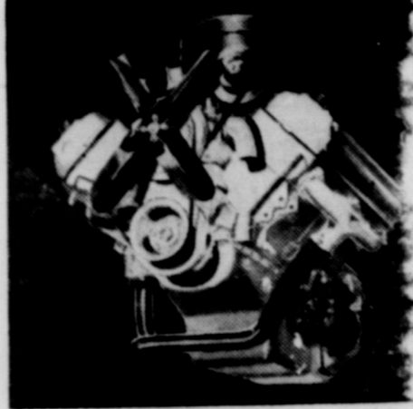
View of the new Chrysler "FirePower" engine. Conservatively rated at 180-horsepower, the new 8-cylinder powerplant is a 90-degree valve-in-head V-type engine.
