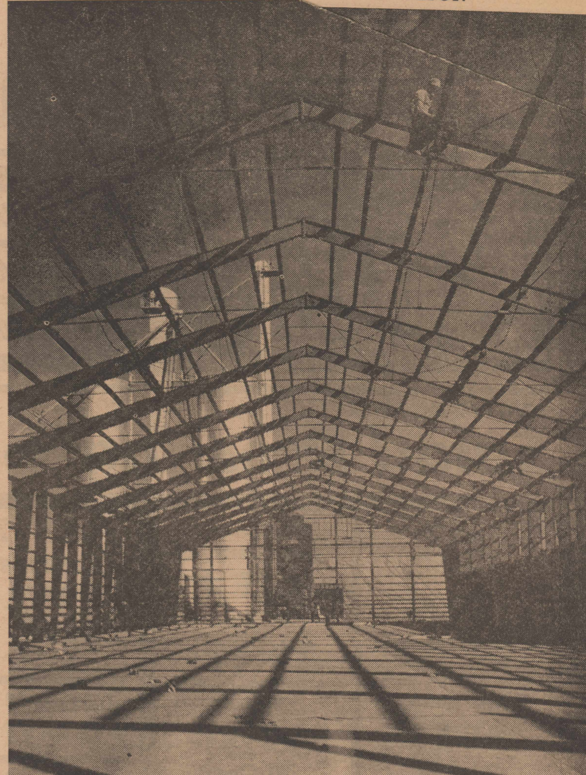
Construction of Olton Grain Elevator's new storage unit is shown in the process of being completed. The structure, being erected by Panhandle Steel Buildings, looked like this during construction.
