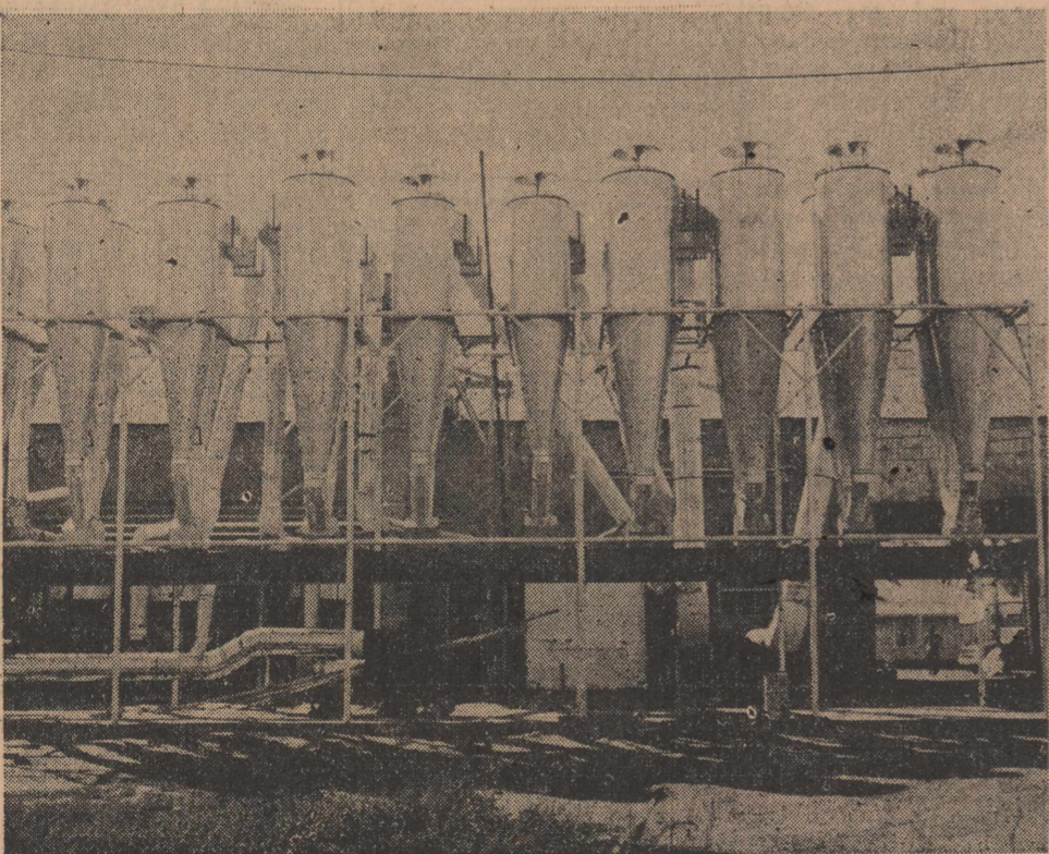
22 CYCLONE DUST, LINT AND AIR COLLECTORS
