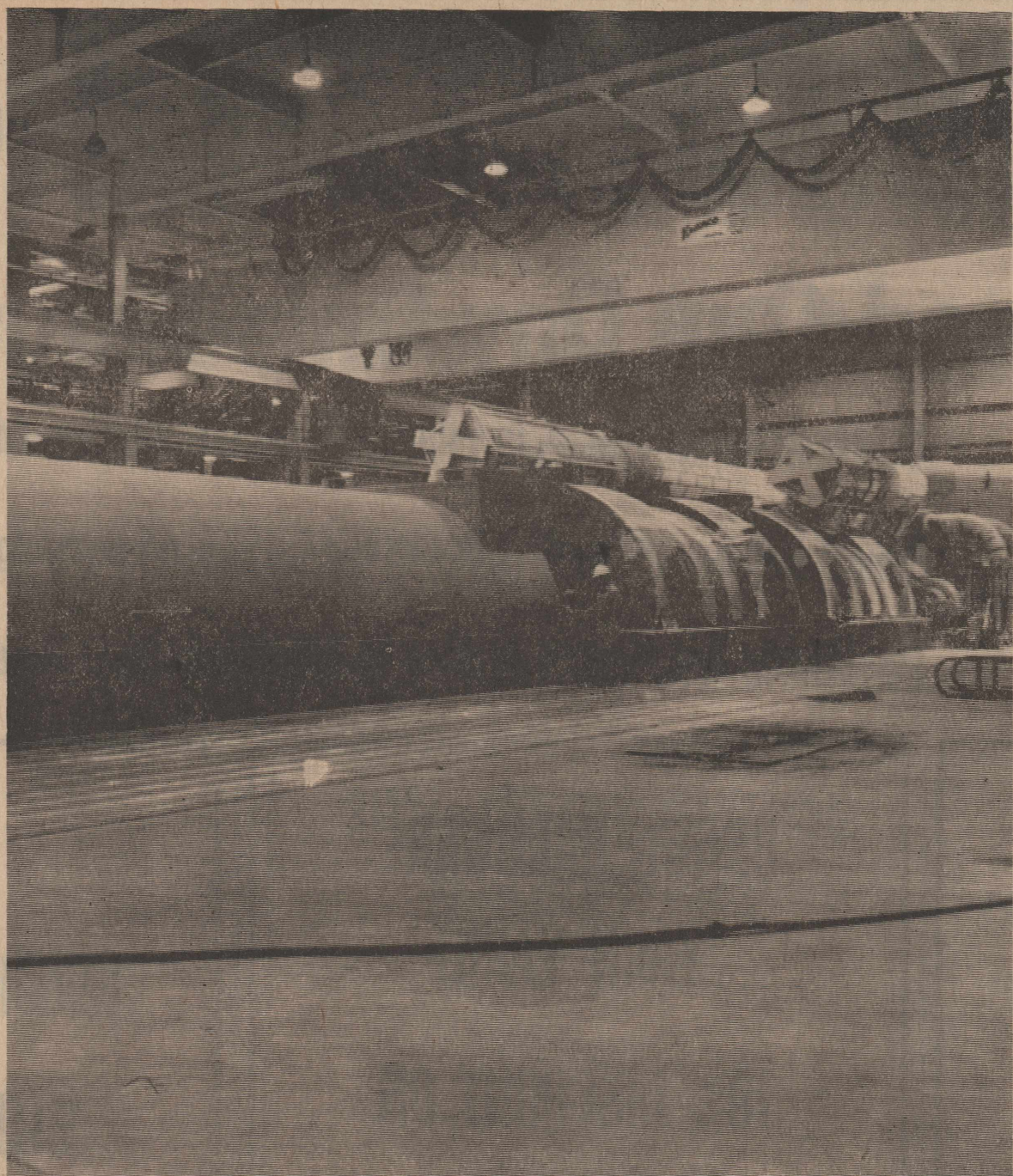
Steam drives this enormous turbine-generator at Southwestern Public Service Company's coal-fired Tolk Station Unit No. 1. The generator stator alone (the unmoving part of the generator) weighs 636,000 pounds. The generator can produce 561,000 kilowatts—enough electricity for 225,000 people. Above the still unpainted turbine is a movable hoist which can raise and lift out all the parts of the turbine generator for periodic maintenance. Among those who toured the facility last Friday were Lee Clay, Stan Fogerson, A. R. Martin, David Tipton, Jerry Patton and Charles Sarchet.
