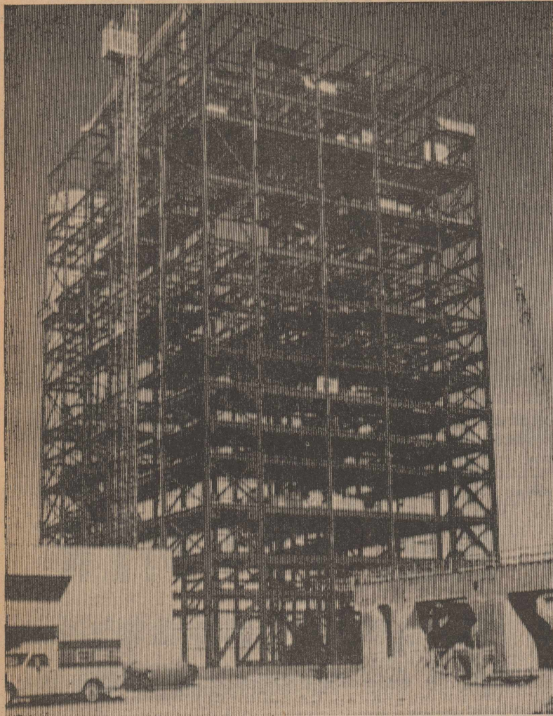
Harrington Station, Southwestern Public Service Company's first coal-fired generating station, northeast of Amarillo, is scheduled for completion in mid-1976. The new 350,000 kilowatt generating facility is a part of the $345-million expansion and improvement
