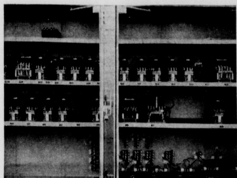
"LIFESAVERS"—This electronic equipment plays its part in helping save lives at railroad crossings. These relays and other units are housed in a large metal cabinet mounted between sets of railroad tracks just south of FM 2060 near the Santa Fe depot. They operate the red-flashing lights and bell-changing devices that warn motorists of approaching trains at the new FM 2060 crossing. (Rev-Foto)
