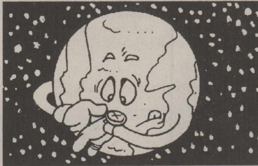
Because of friction caused by tides, the Earth's rotation slows and the day increases about a millisecond each century.
