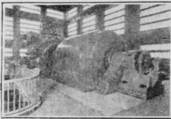
The Largest Turbo-Generator in the South Capacity 30,000 K. W. One Third as Large as Unit Being Installed on East River in New York
