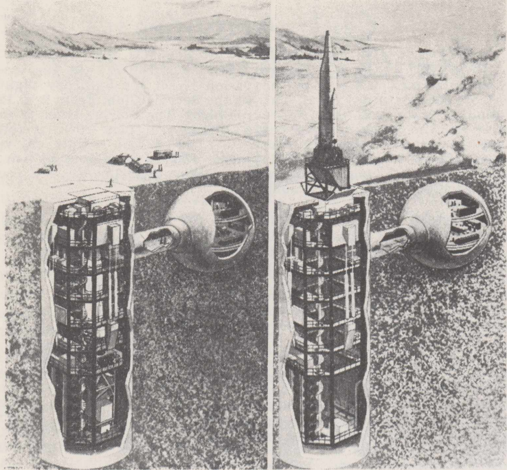
UNDERGROUND ATLAS —Silo emplacement of the Air Force Atlas intercontinental ballistic missile will resemble this artist's conception of hardened Atlas squadrons. At left, maintenance, checkout and fuel operations are carried out underground in the silo containing the missiles. At right, Atlas has been raised and its rocket engines lighted. Countdown of the big missile is conducted in spherical underground blockhouse at right of silo.
