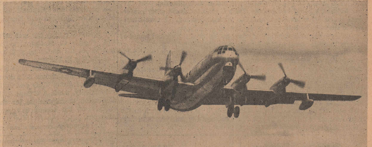
TURBOPROP—The Boeing YC-97I, one of two Stratofreighters which will serve as test bed for the new Pratt & Whitney T34 engine is shown taking off on its maiden flight April 19. The airplane remained in the air for one hour and 15 minutes on its first flight.
