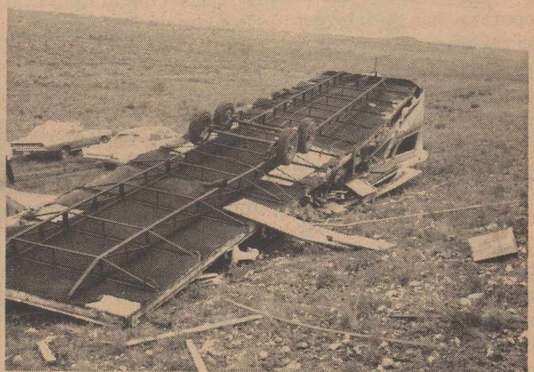
This picture was taken from the upper side and the complete running gear and frame is shown. Note the debris in the foreground. (The H. B. Patterson, Jr. home can be seen in the background.)
