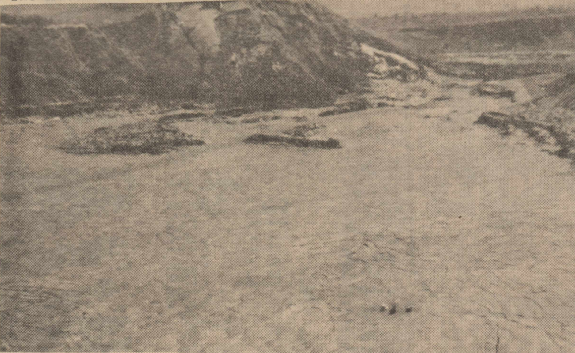
It is 11.1 miles around this crater, 4 across, it shot 1900 ft. in the air when it was making new rock. Notice the Seismograph station out in the middle.
