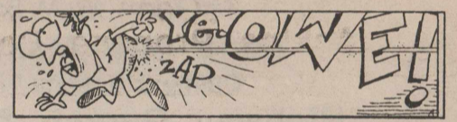
The word laser stands for light amplification by stimulated emission of radiation.
