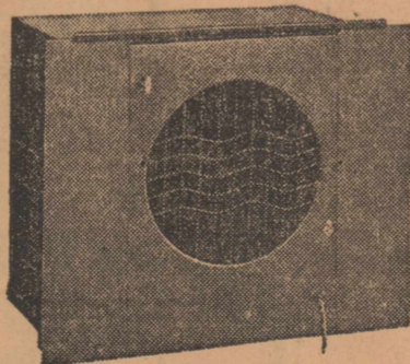
STANDARD MODEL
