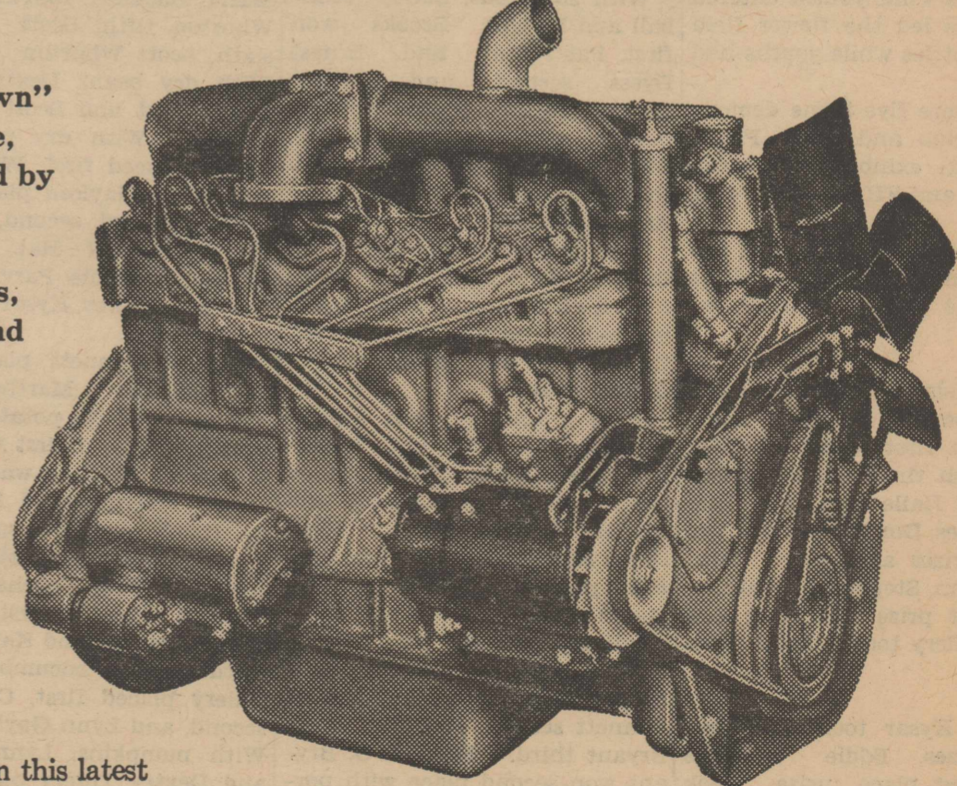
International D-301 Engine gives you low-cost diesel performance for the short haul. Naturally aspirated 301 cu. in. engine delivers 110 hp. at 3,000 rpm. Weighs only 902 lbs. or 8.2 lbs. per horsepower. High torque output at low speed, low fuel consumption and long life between overhauls have been proven in actual truck use. Direct electric starting and a simplified fuel system are other advantages. Heavy-duty construction features include fully-hardened crankshaft and reinforced crankcase.
