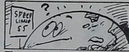
The speed of the earth's spin slows about a second a century.
