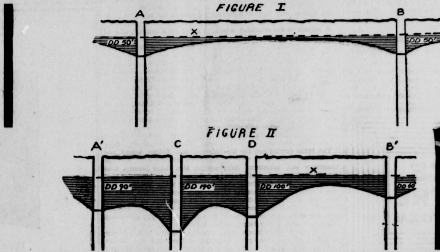
Figure 1. Water level at proper spacing. Figure 2. Water level at improper spacing.
