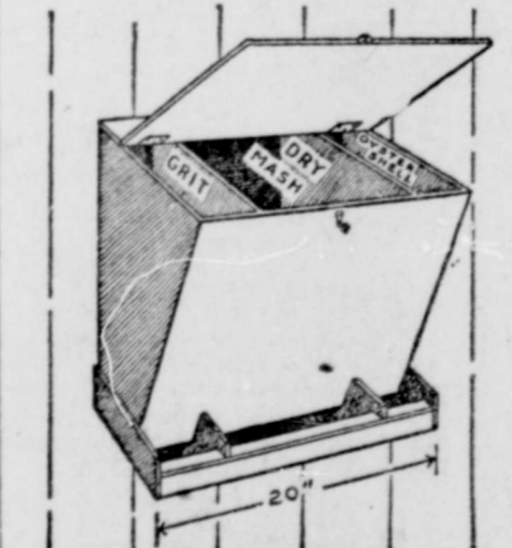
Dry-Mash Hopper for Use in the Laying House.
