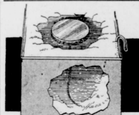
Sectional view of typical de-icer installation.
