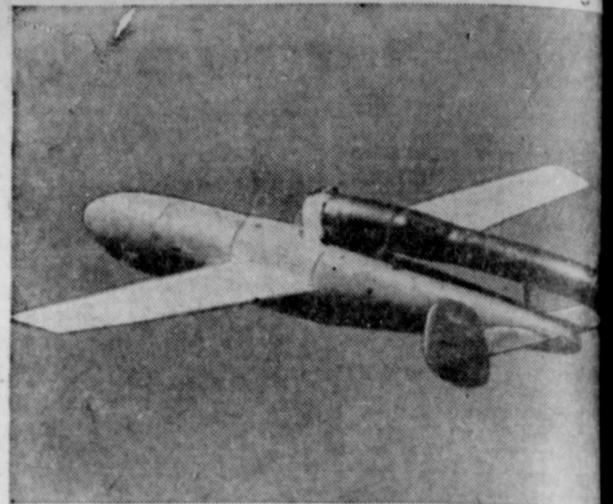
SHOWN IN FLIGHT over Washington, this pulse-jet powered pilotless craft target of the U. S. Navy is to be used for training naval gunners. It resembles the German "buzz bomb" of the late war. Known as the KD2G-2, it is remotely controlled from air or land. With mission completed, it can float down by parachute. (International)
