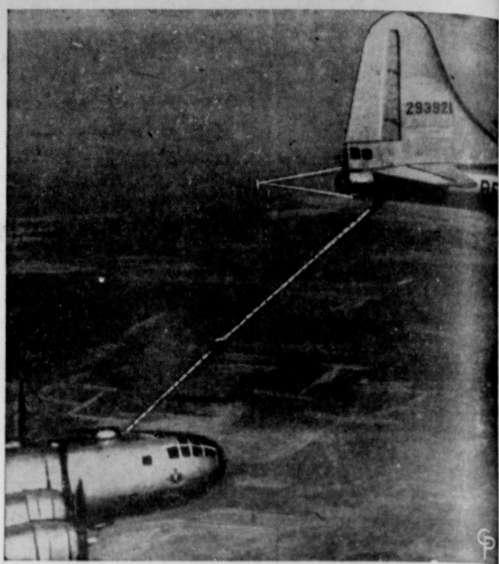
IN MID-AIR a B-29 tanker (top) makes contact with B-29 bomber in new type plane-to-plane refueling operation over Seattle, Wash. Fuel is transferred under pressure through "flying boom" developed for the Air Force by Boeing aircraft. (International Soundphoto)
