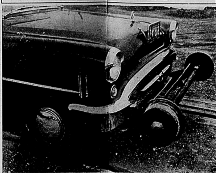
This specially-equipped Buick, one of 13 used by the Chicago, Burlington and Quincy railroad, is equally at home on highway or railroad. The dual-purpose car is fitted with front and rear flanged wheels, shown here in raised position for highway operation. The wheels can be lowered hydraulically for use on the railroad tracks, with the regular rear wheels providing traction. The Burlington uses its fleet of eight-wheeled Buicks for inspection of branch lines, going across country via highway from the end of one spur to another.
