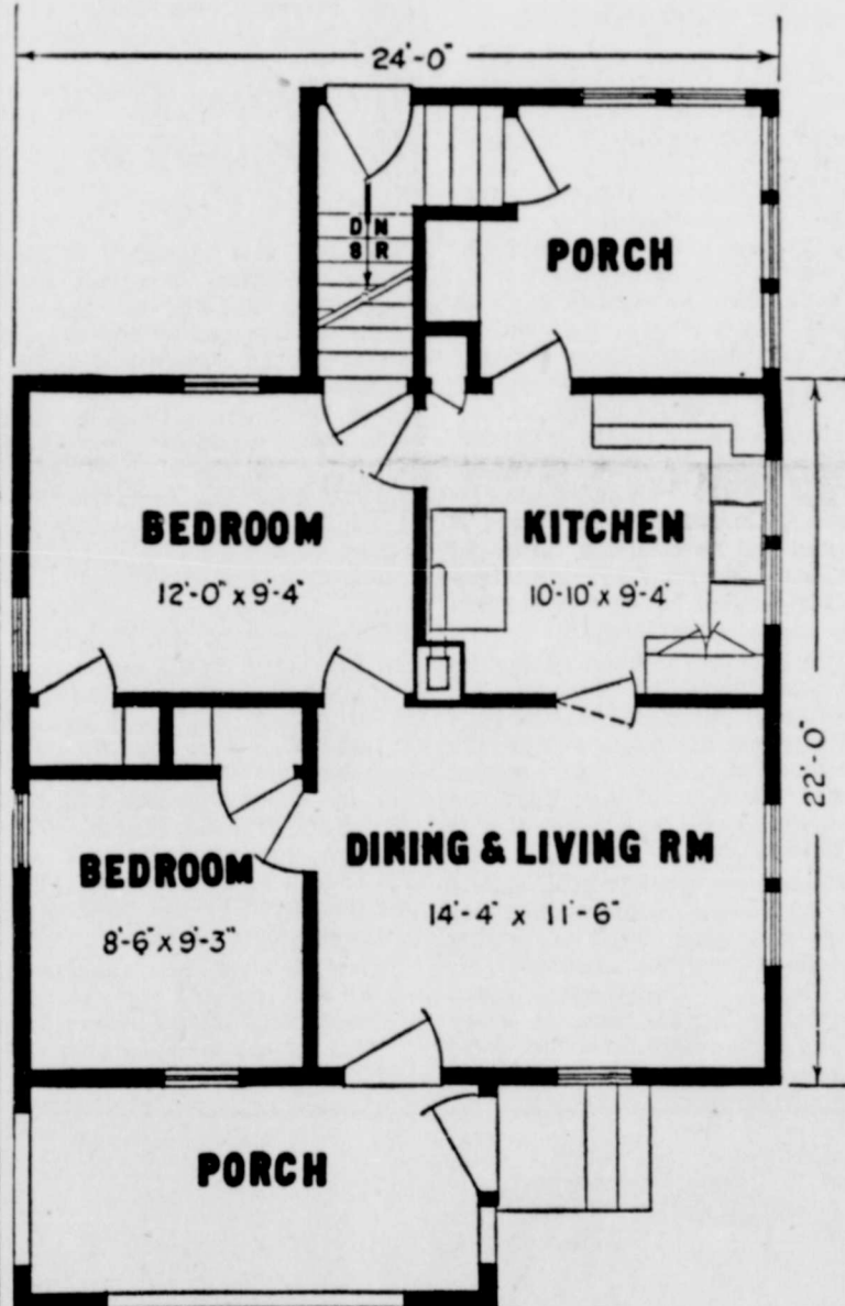
Floor plan of four-room farmhouse
