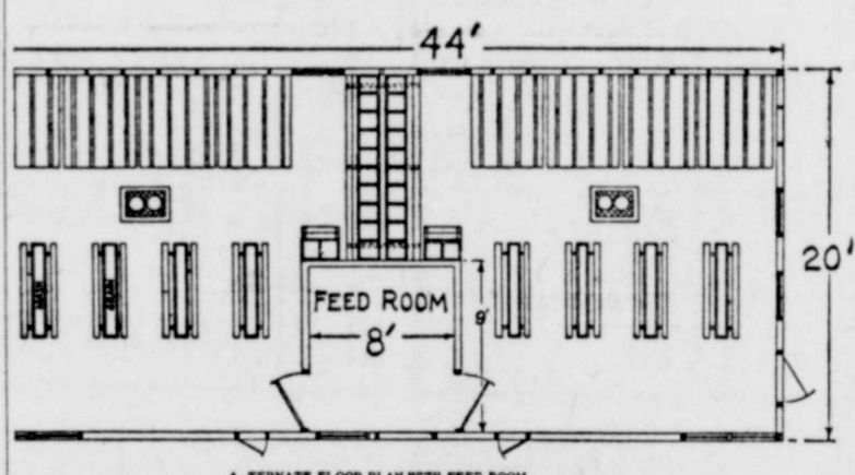
A. TERMINATE FLOOR PLAN WITH FEED ROOM
