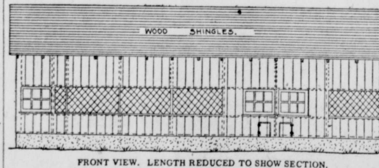
FRONT VIEW. LENGTH REDUCED TO SHOW SECTION.
