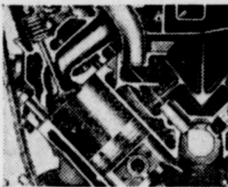
New Ford LOW FRICTION design truck engines have short piston stroke, therefore less friction drag, wear and heat, more delivered power! New overhead valves!
