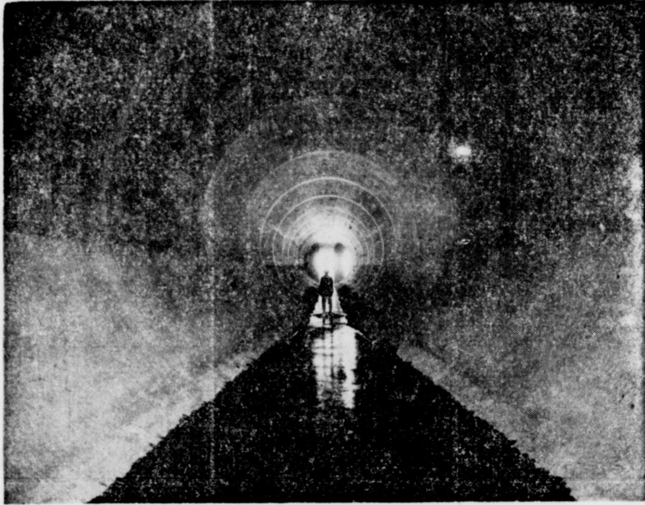
BIG TUBE —This is one of the two circular discharge conduits that will control the flow of water from behind the North Concho Dam, San Angelo's $16,200,000 flood-control project. Each of the tubes is 18 feet in diameter. Height of the six-foot workman wading through the tube gives some idea of their tremendous size.
