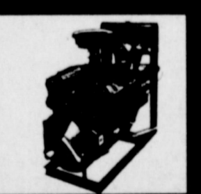
C-605 Hundreds of pounds heavier and a higher 9.5:1 compression ratio makes this big 605 CID truck engine superior to any competitive model in both power and fuel economy.
