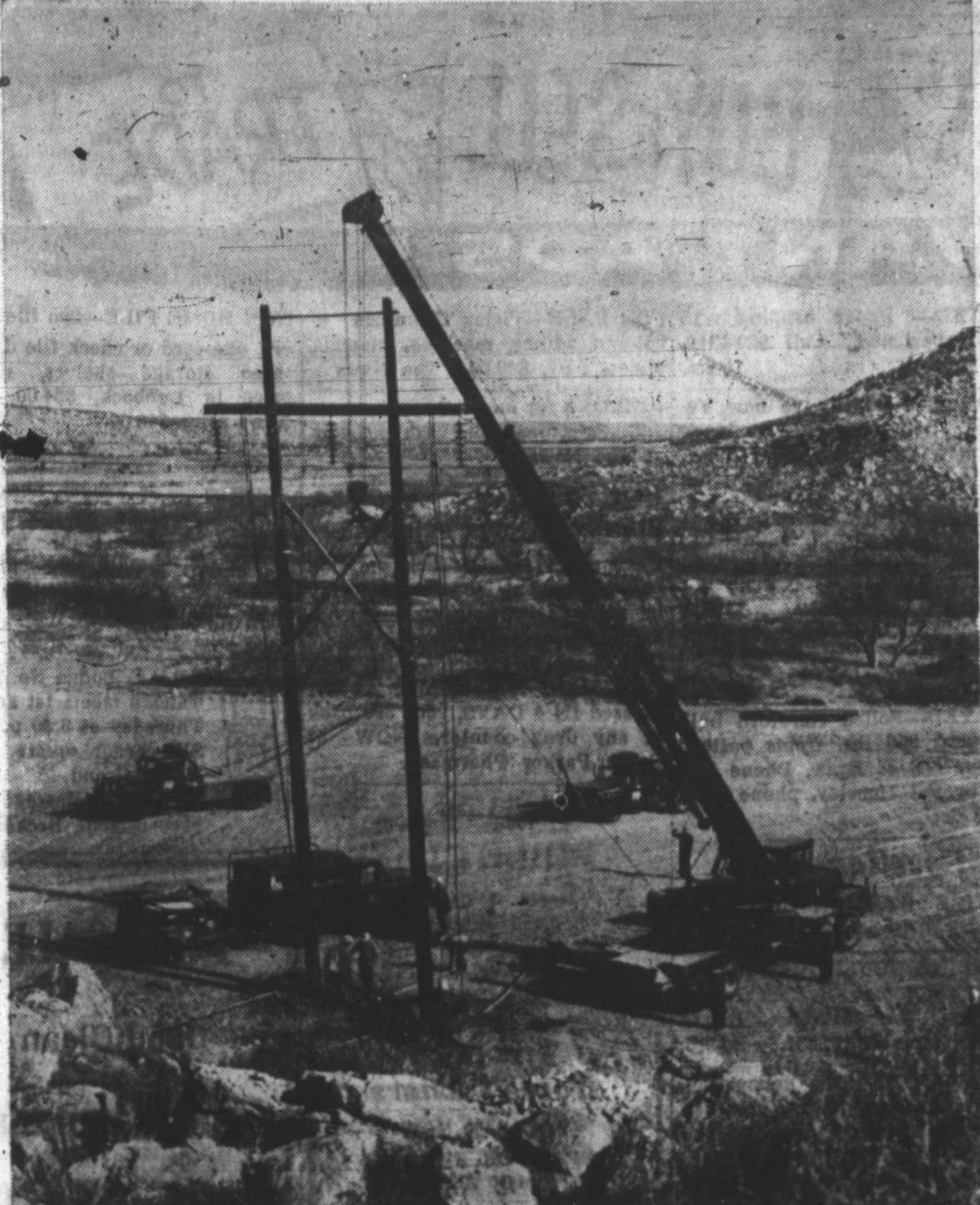
AN 80 FOOT electric transmission line structure can be lifted and set into place in 8 1/2 minutes with Southwestern Public Service Company's new hydraulic crane. The unit, the second one to go into service in the nation, was specifically designed for use in the electric utility industry. Southwestern Public Service Company has announced a 1966 construction program calling for the investment of $19,353,000 in new facilities, with a large portion of the additional investment to be in transmission lines.
