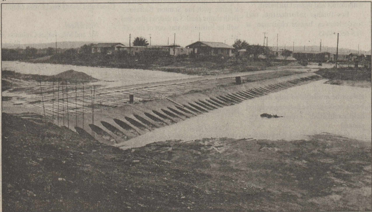
WATER WENT THROUGH THE CULVERTS Monday at the low water crossing being built across Johnson Draw at War Admiral Street. The project is expected to be completed in November. Photo by Stephen Zuberbueller
