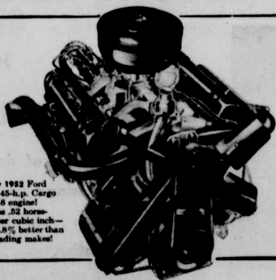
New Ford LOW FRICTION design truck engines have short piston stroke. Therefore less friction drag, wear and heat, more delivered power! New overhead valves!
