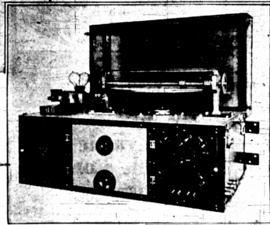
The hills and dales, mountain crests and chasms of the ocean are measured by this device, which enables the geographer of the sea's floor to accurately figure distances.
