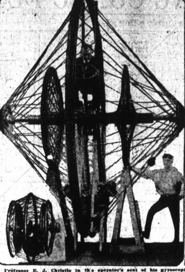
Professor E. J. Christie in the operator's seat of his gyroscopic unicycle racing car.
