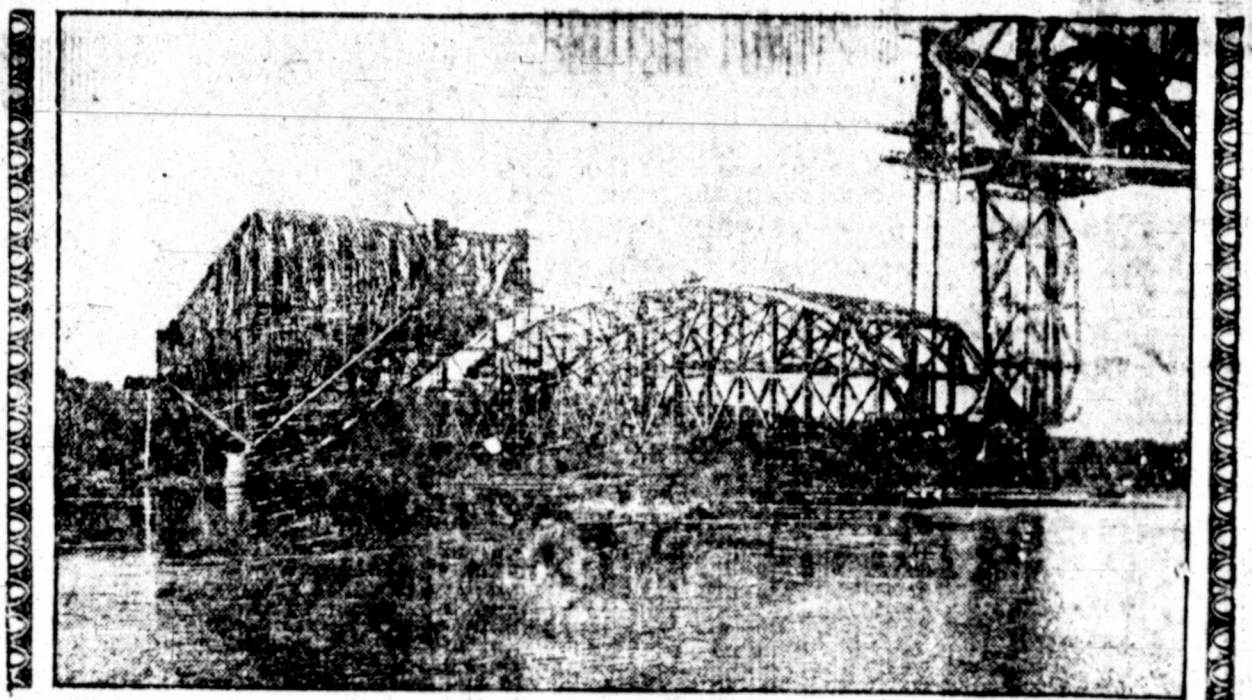
One year after the fatal accident at the big Quebec bridge another attempt to raise into place the center span that fell was made, and it was successful. The span is 122 feet above the St. Lawrence river. It is 640 feet long and was brought down the river to the bridge site on pontoons. It was suspended from the opposite ends of the bridge by chains and raised into place by powerful jacks.
