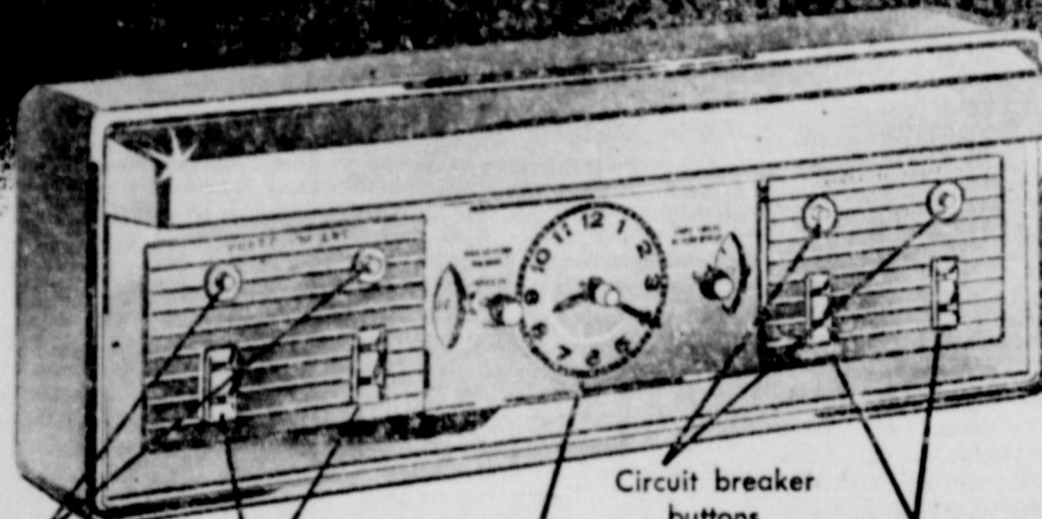
Circuit breaker buttons, 110-volt outlets, Timer clock for automatic cooking, 110-volt outlets (one timed)
