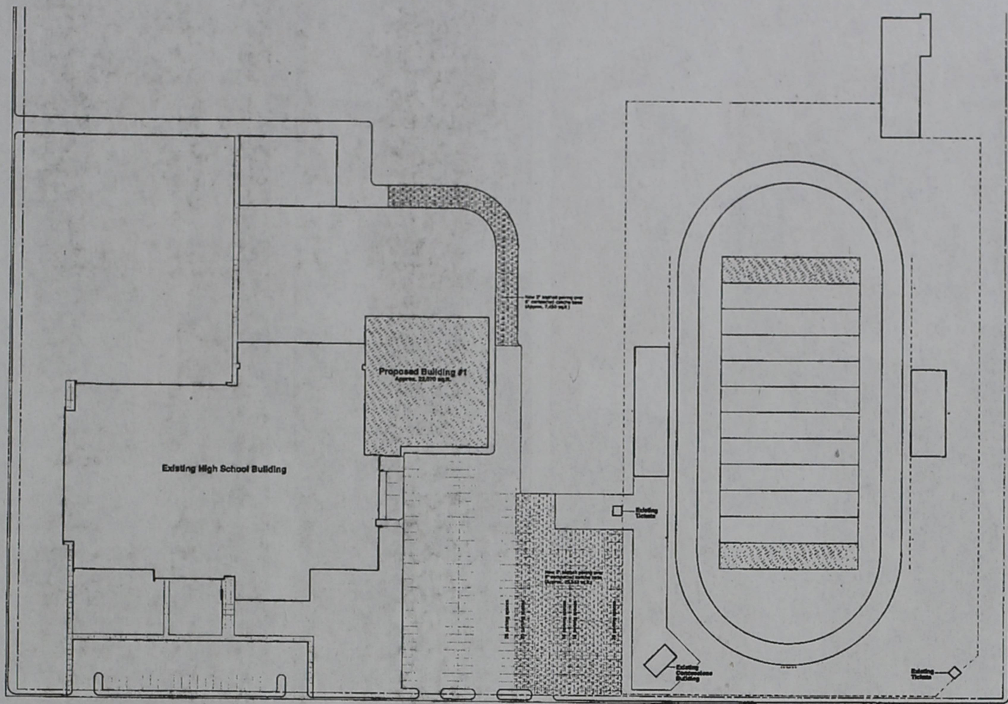
Friona Independent School District High School Auxiliary Gym Project Proposed Site Plan #1
