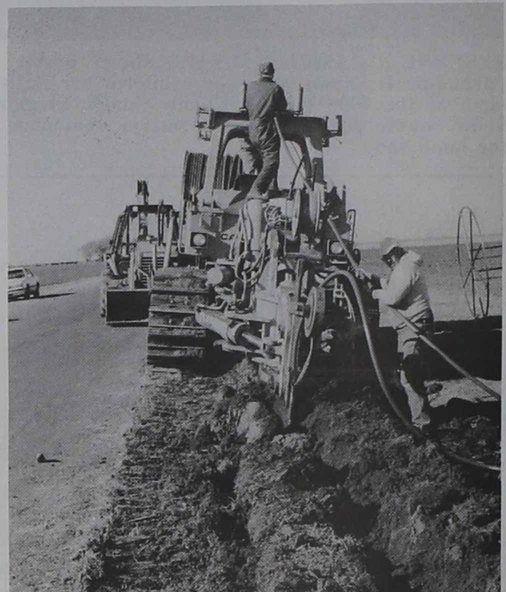
INSTALL CABLE... Crew members from Brooks Construction Company, contractor for a cable-laying project for West Texas Rural Telephone Cooperative, are shown at work on installation of a stretch of cable that's part of the 40 miles of fiber-optic cable being buried by the cooperative in an ambitious upgrading project in Parmer, Deaf Smith and Castro counties. Upon completion of the project, all of WTRT's central offices in Parmer, Deaf Smith and Castro counties will be linked by fiber-optic cable. (WTRT Photos)
