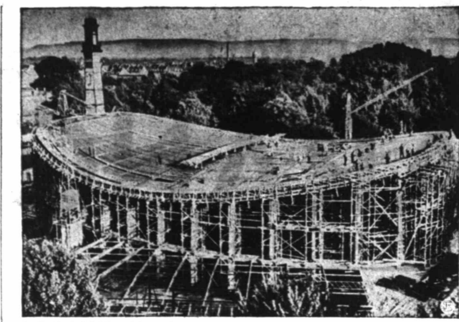
THIS IS A ROOF?—This saddle-shaped hanging roof of the "Black Forest Hall" in Karlsruhe, Germany, will have no center supports. Concrete pillars spaced throughout the glass walls will support the unique three-inch-thick steel and concrete roof.
