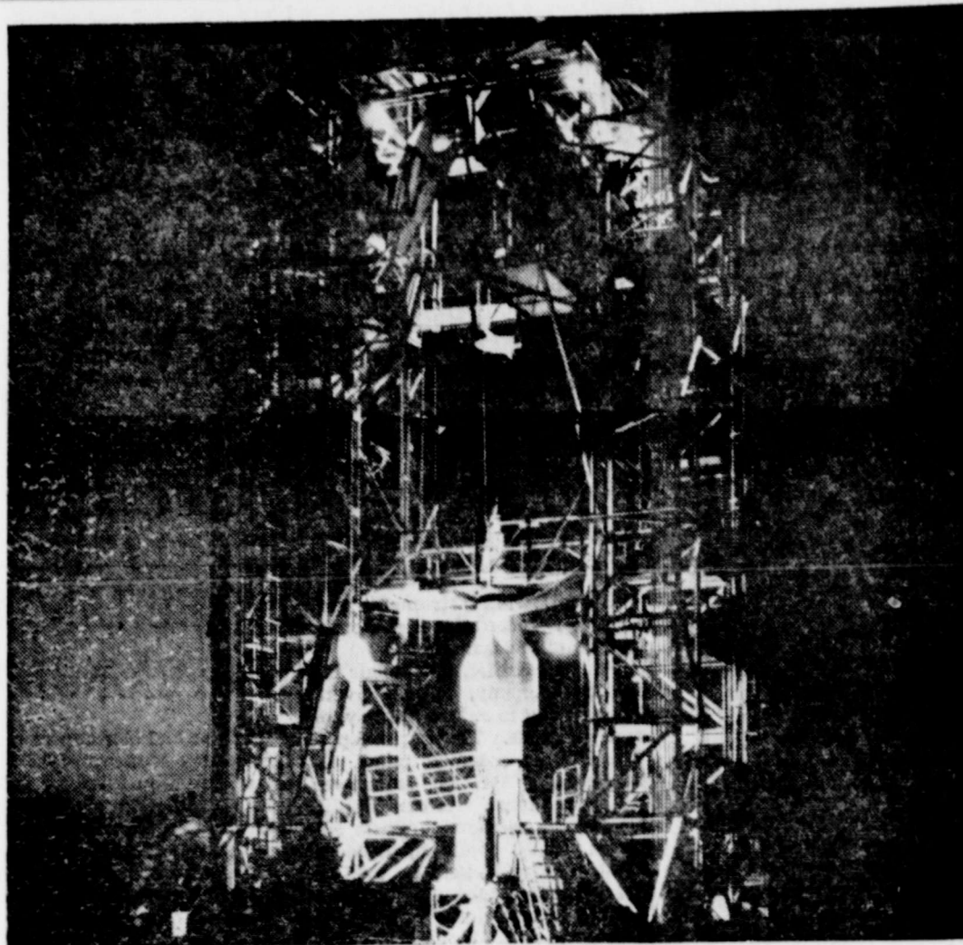
EXPLOSIVE BEAUTY —Hermes guided missile—named after the wing-footed messenger of the god in Greek mythology—is readied for test firing at the Army's White Sands Proving Ground, N.M. Project Hermes is a joint venture by the Army Ordnance Corps and General Electric Company. It was initiated to produce missiles both as weapons and for research in the upper atmosphere.
