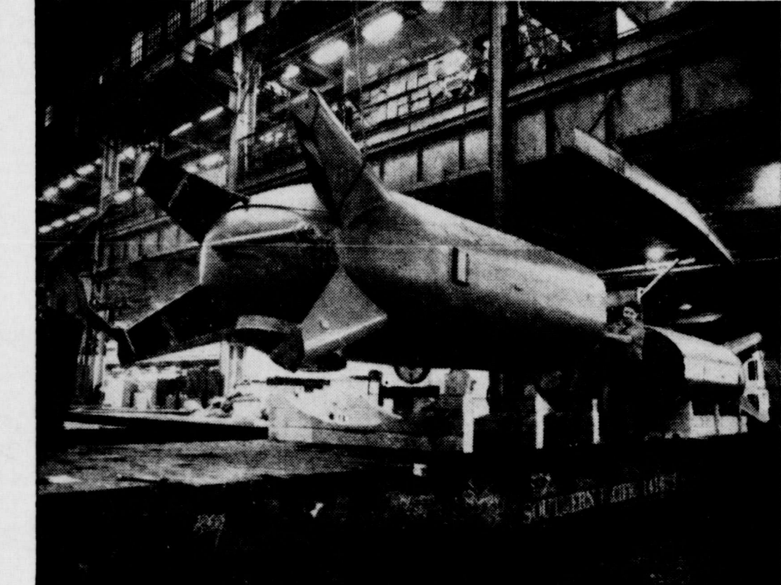
FOR THE ATOMIC CAUSE—Because of its size, a three-pole circuit breaker built in East Pittsburgh, Pa., for an atomic plant in Ohio, had to be disassembled for shipment on railroad flat cars. This is the first of 35 which will be built. With an interrupting capacity of 25 million kilovolt-amperes, a single breaker can control the electric power of a large city.
