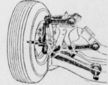
Ball-Joint Front Suspension It allows greater up and down wheel travel for a smoother ride... helps keep wheels in true alignment for consistently easy handling. Wheels move on ball joints, whether up or down... right or left.
