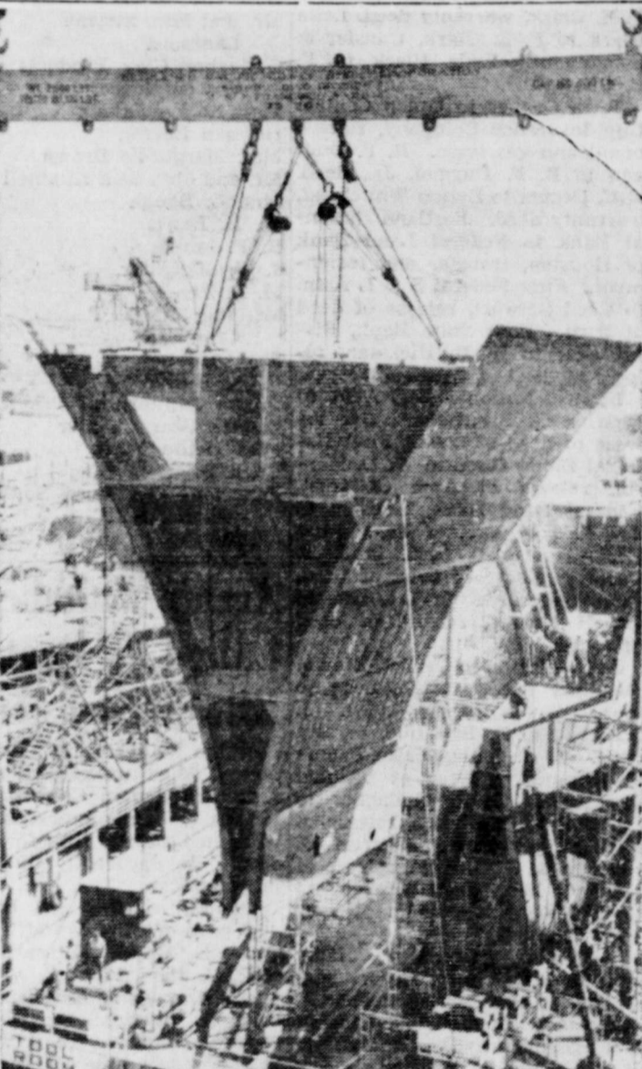
SHIP-SHAPING —Construction of the SS Golden Mariner, one of five high-speed cargo ships being built at San Francisco, makes a big stride toward completion as two giant cranes ease a 70-ton prefabricated section of the bow into place. Once lowered into position, the steel unit was shored up and welded to the hull structure. Launching is expected this fall.
