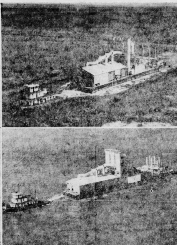
building costs of a permanent plant were prohibitive. The 65-mile trip from Grand Ecaille, where the plant was assembled, to Bay Ste. Elaine was in itself an outstanding engineering feat which required split-second timing. Top photo shows the plant being towed through a bayou and, below, the towing tug is just entering Timberlier Bay, near the Gulf of Mexico.
