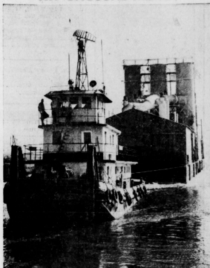
FLOATING GIANT —American industry reached a new milestone with the moving of the world's only floating sulphur mining plant 65 miles to its mine site at Bay Ste. Elaine in the Louisiana bayou country. The unusual plant, shown setting out, was built by Freeport Sulphur Company to solve the engineering problem of extracting sulphur from a marshland where
