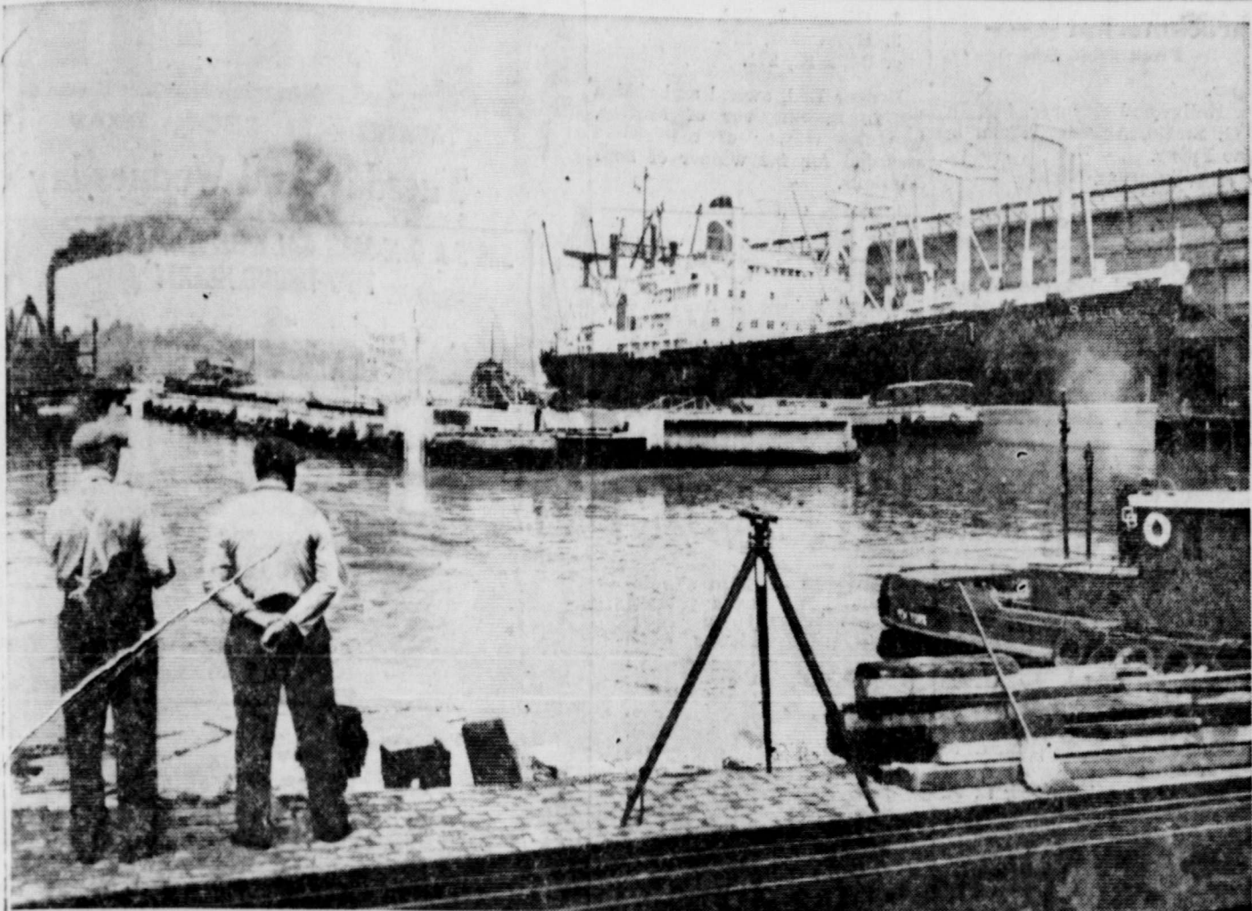
FLOATING IT IN —The first of three huge concrete sections that will form the foundation of a new pier along the Hudson River in New York arrived after six tugs pulled it 38 miles. The 367-foot long, 80-foot wide, 26-foot high caisson is the smallest.
