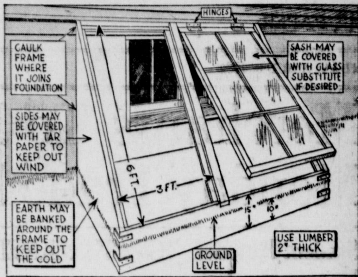
Working Drawing for Hotbed Outside Basement Window.
