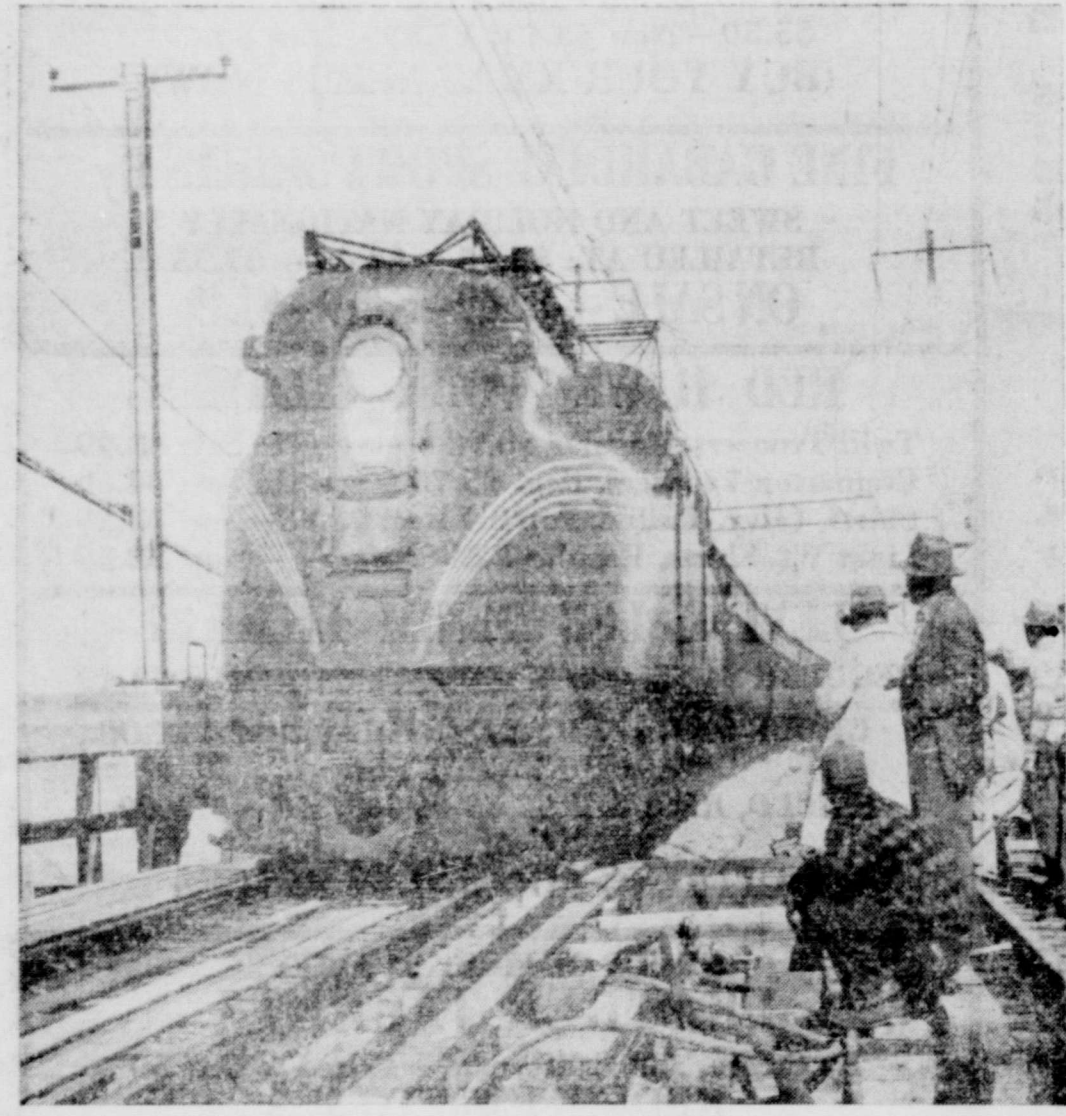
SOMETHING'S GOT TO BE FIRST —And this train, rolling over the Pennsylvania Railroad span at Woodbridge, N.J., is the first to cross after the final check on the new 200-foot structure. It took workmen 12 hours to put the 2000-ton span in place and lay the rails.
