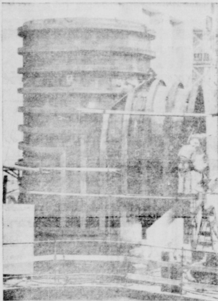
SLIGHTLY OVER-SIZE —A workman welds together sections of a giant pressure relief valve discharge liner being installed at the power plant at Hoover Dam on the Colorado River. It weighs 65,000 pounds, stands 26 feet high and is 14 feet in diameter. The liner's bulk had to be shipped in sections.
