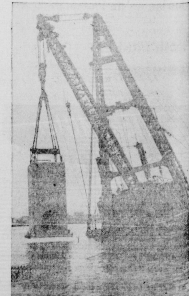
GETTING INTO POSITION —A 200-ton box of reinforced concrete that will serve as the outfall chamber for Nassau County's new sewage treatment works is lowered into position by a floating derrick in New York. The chamber is 29 feet 15 feet long and 13 1/2 feet wide. Approximately 8,000 feet of pipeline have also been laid.
